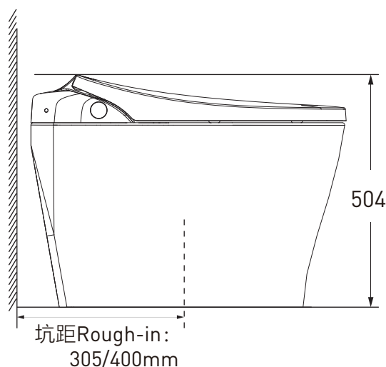
侧面图 Side View
