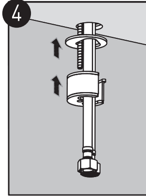
产品有单杆固定或双杆固定 Product may have either one or two mounting studs
