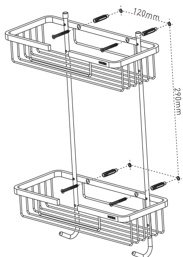
90133 双层置物篮
